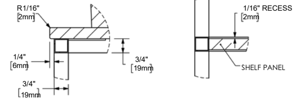
DETAIL BC 1:4
